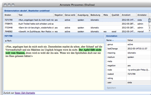
Figure 5: User interface for annotating phrasemes
